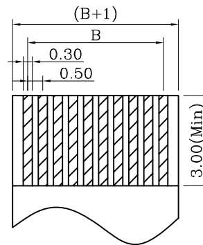
THICKNESS:0.30±0.05 FPC DIMENSION REFERENCE
